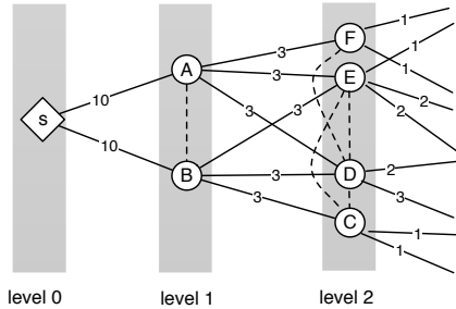
Figure 1: The ticket distribution process of a particular node S : The numbers on each link represent the number of tickets propagated via that link. The dotted lines are links between nodes at the same distant to the source
