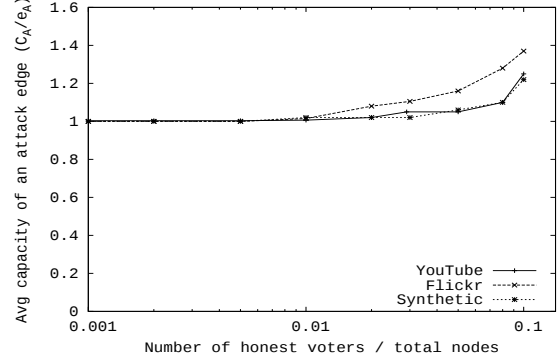
Figure 4: The average capacity per attack edge as a function of the fraction of honest nodes that vote. The average capacity per attack edge remains close to 1, even if 1/10 of honest nodes vote.
