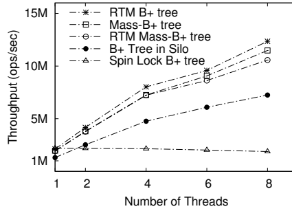
Figure 6: RTM B^+ tree vs. Fine-grained lock-free B^+ tree in masstree (YCSB)
